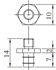
EN-PC-10~20-M5
