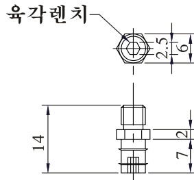
PC-10~20-M5
