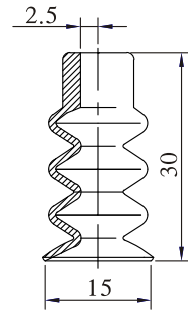
PCCE-15
